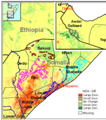
Normalized Difference Vegetation Index (NDVI) Absolute difference w.r.t previous year (Act.—Prev.) for Dekad III of August 2005
