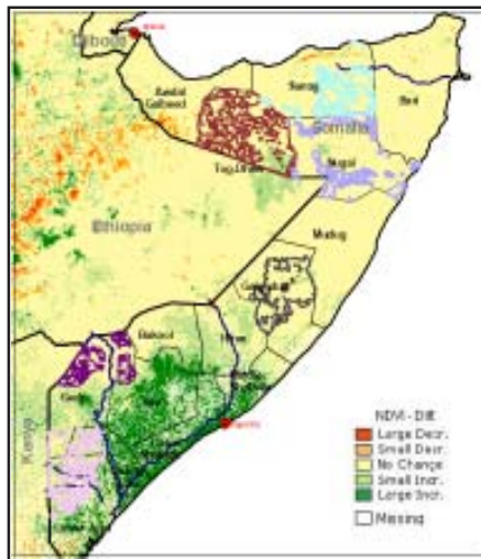
Normalized Difference Vegetation Index (NDVI) Absolute difference w.r.t previous year (Act.—Prev.) for II Dekad
