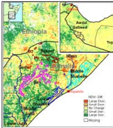
Normalized Difference Vegetation Index (NDVI) Absolute difference w.r.t previous year (Act.—Prev.) for Dekad III of April 2006
