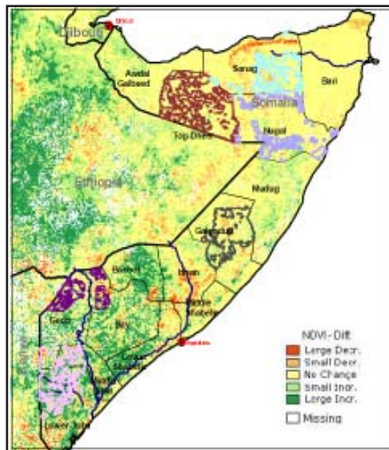
Normalized Difference Vegetation Index (NDVI) Absolute difference w.r.t previous year (Act.—Prev.) for Dekad III of April 2006
