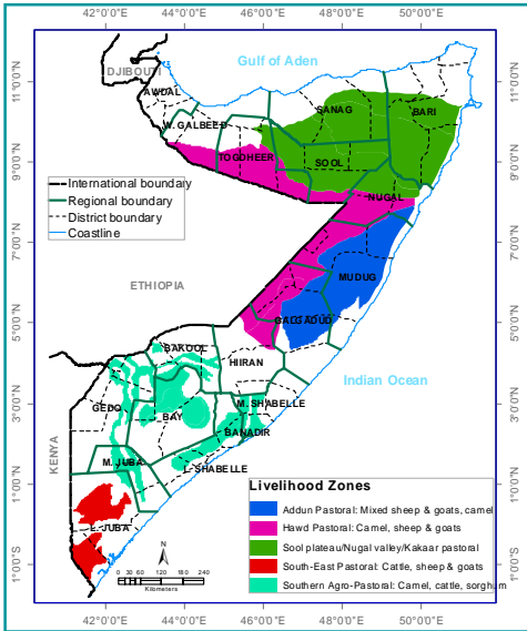
Livelihood Zones Used in Time Series Analysis
