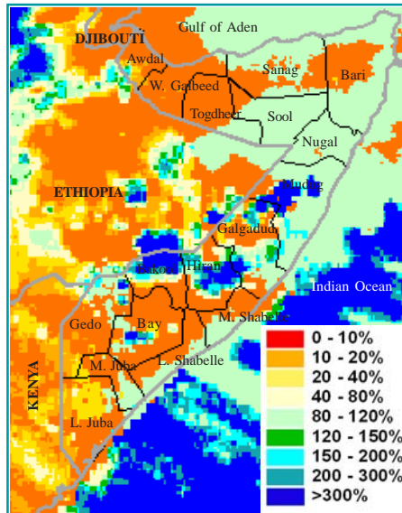
February '07: Rainfall as % of Long Term Mean
