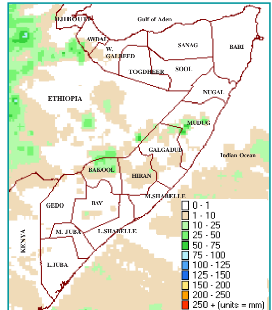
February '07: Cumulative Rainfall (RFE) (mm)
