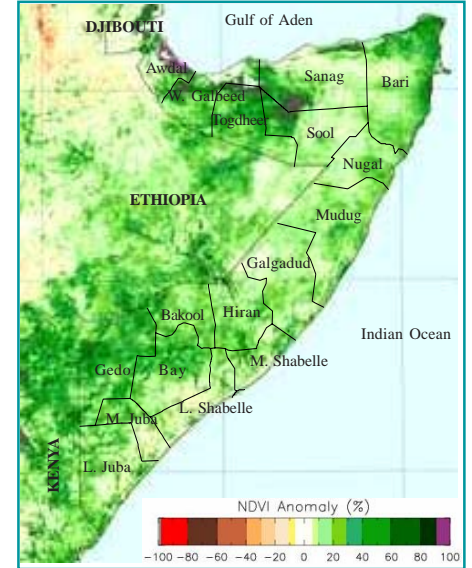
February '07: NDVI, as % of Long Term Mean
