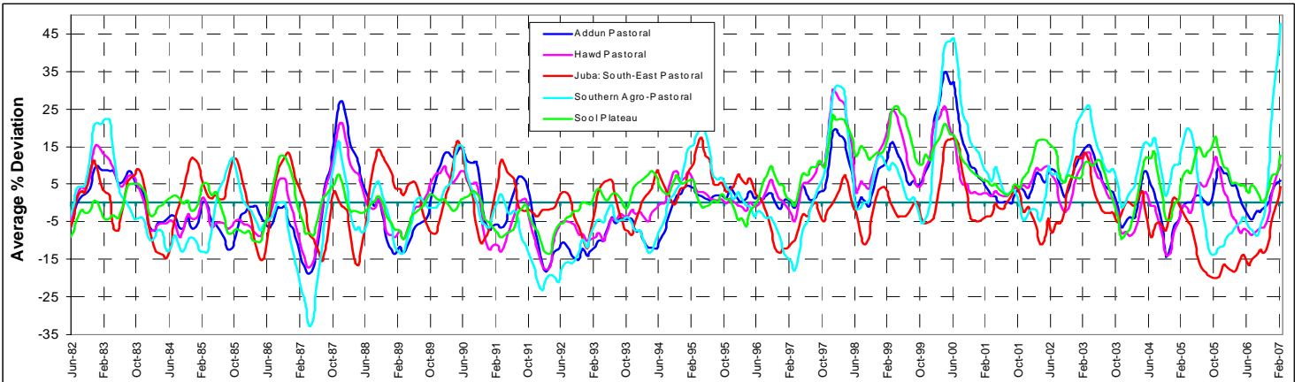
Historic RFE % Deviation From Long Term Average
