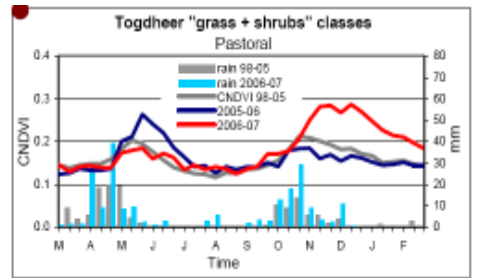
February '07, 3rd Dekad
