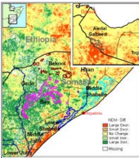
Normalized Difference Vegetation Index (NDVI) Absolute difference w.r.t previous year (Act.—Prev.) for Dekad III of May 2006
