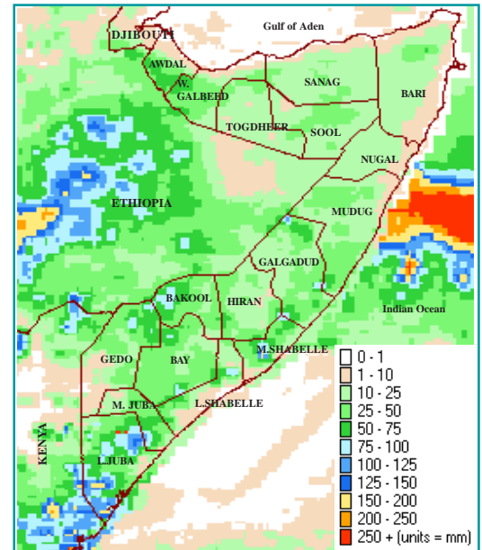
April '06: Cummulative Rainfall (RFE) (mm)
