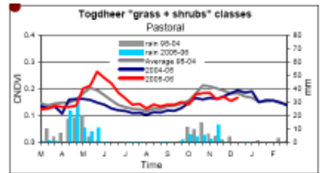
December 11-20 II Dekad
