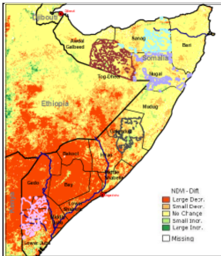
Normalized Difference Vegetation Index (NDVI) Absolute difference w.r.t previous year (Act.—Prev.) for Dekad II of December 2005
