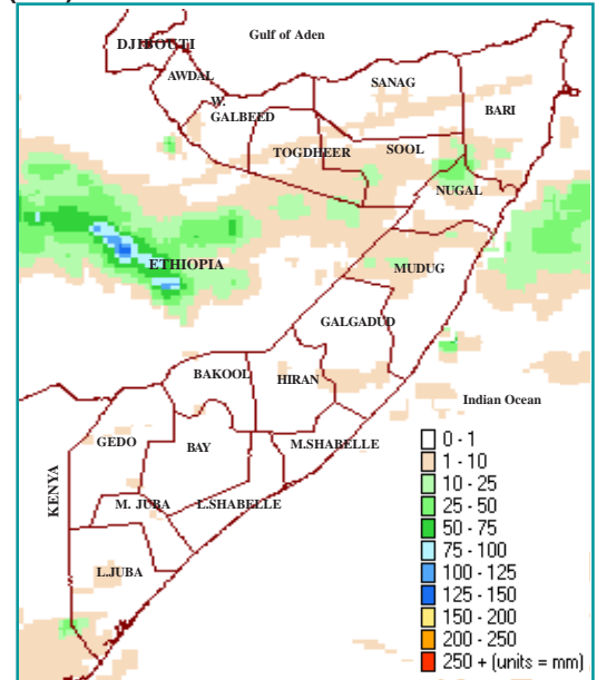
December '05: Cummulative Rainfall (RFE) (mm)
