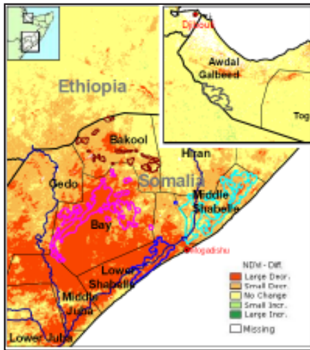
Normalized Difference Vegetation Index (NDVI) Absolute difference w.r.t previous year (Act.—Prev.) for Dekad III of January 2006
