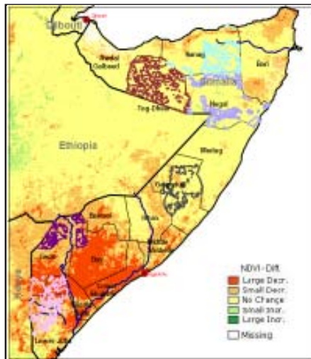
Normalized Difference Vegetation Index (NDVI) Absolute difference w.r.t previous year (Act.—Prev.) for Dekad III of January 2006
